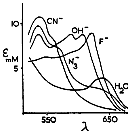
FIG. 4. The absorption spectra of some myoglobin complexes (27)
